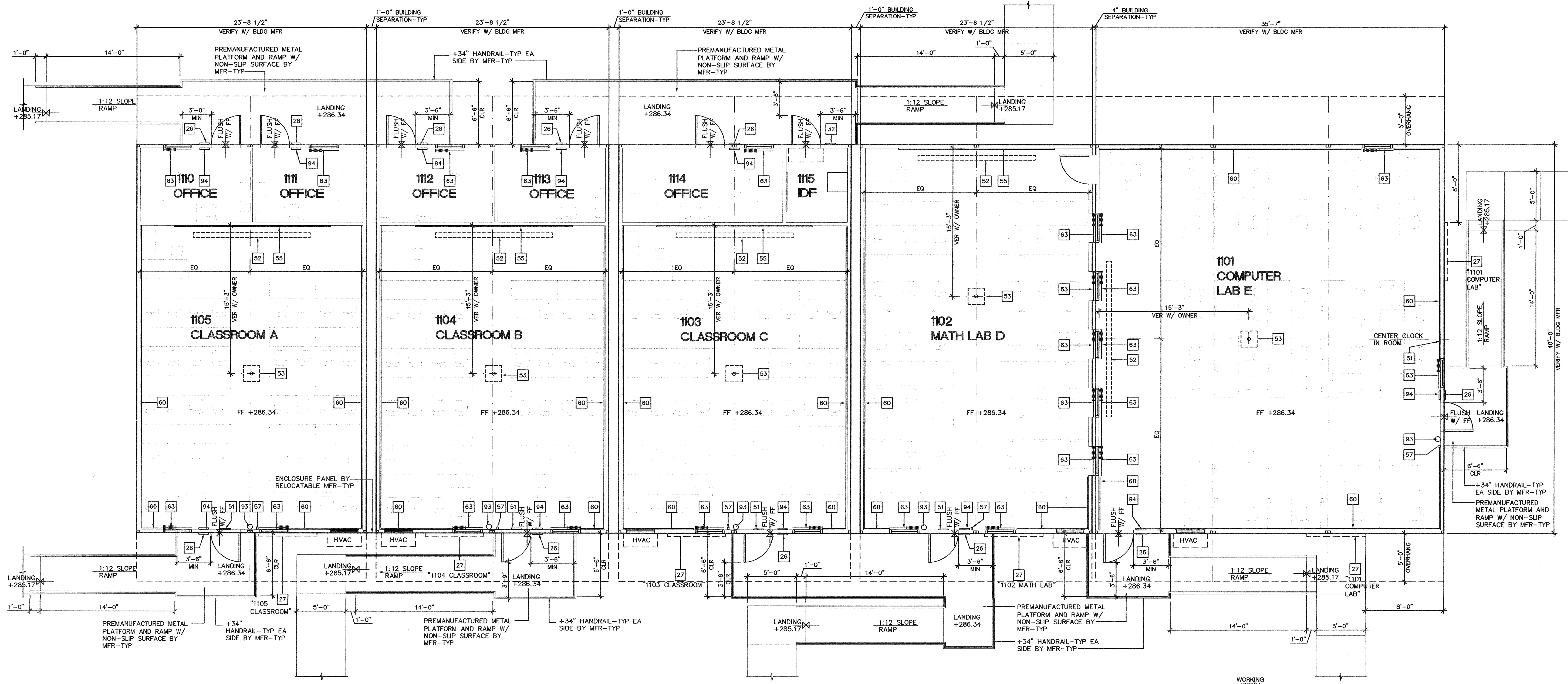
Building 11 Floor Plan 3/16"=1'-0"
