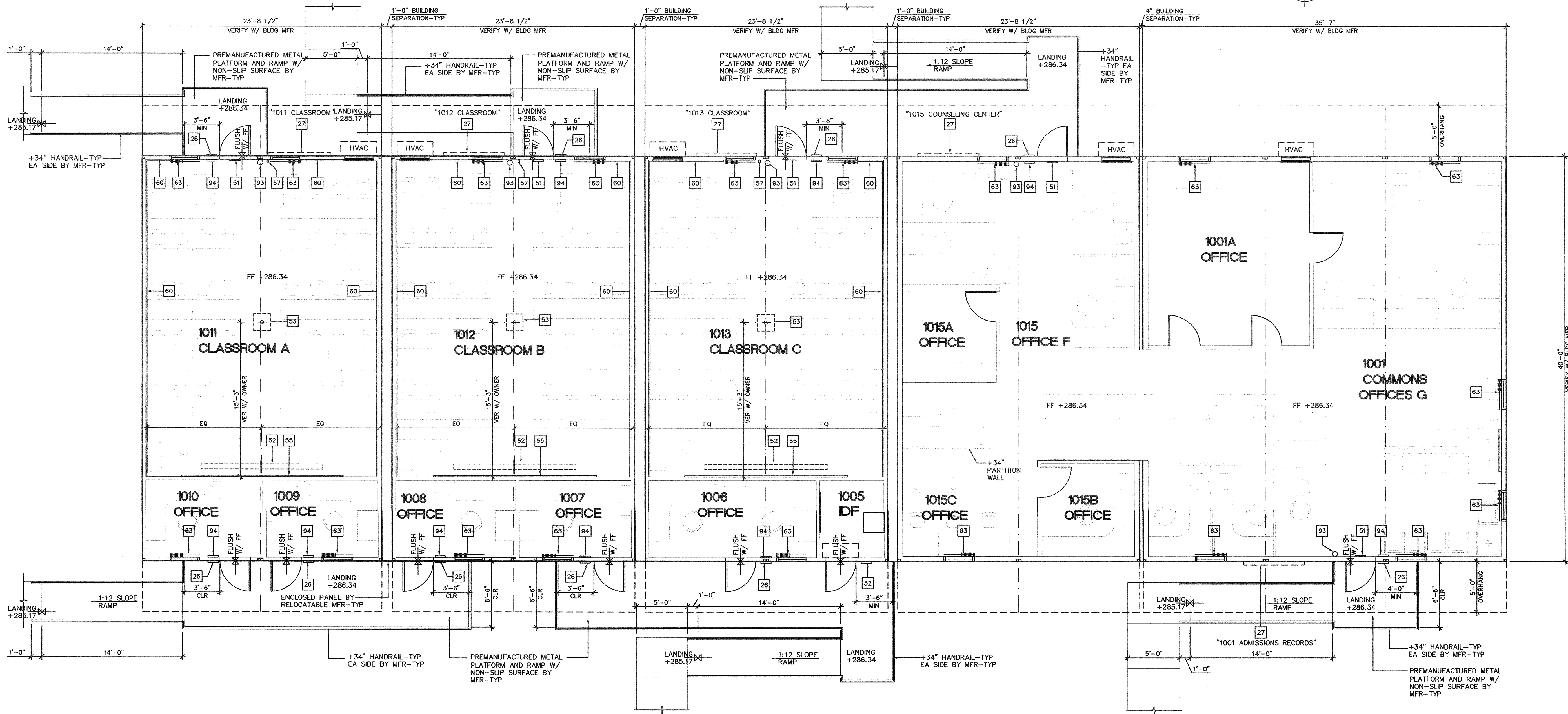
Building 10 Floor Plan 3/16"=1'-0"
